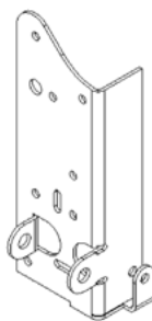
(7) BOTTOM BRACKET (27017) - RIGHT
