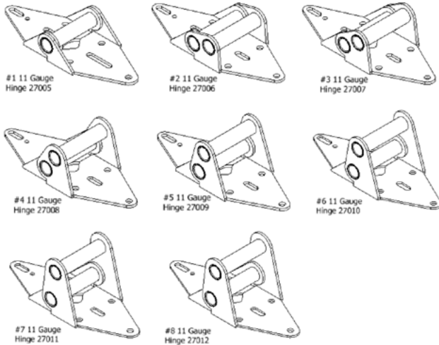
(4) END HINGES #1 UP TO #8 (DEPENDS ON NUMBER OF PANELS) (27005- 27012)
